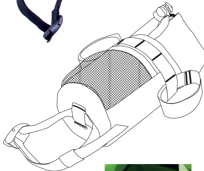
STRAP WITH CAMLOK BUCKLE TO FIX THE BOTTOM TO THE FORK CROWN.
